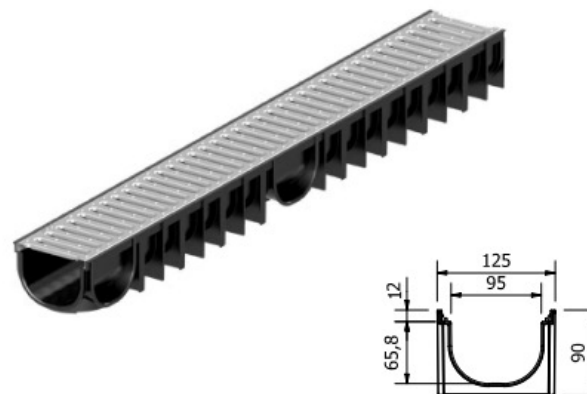
ACO CANAL+REJA 3 CNL EASYLINE 100 HDPE NEGRO H90 L1 REF. 33081810 PVP. 10,65€
