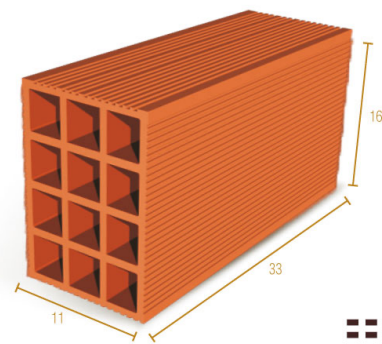
RASILLON TRIPLE 33X16X11
